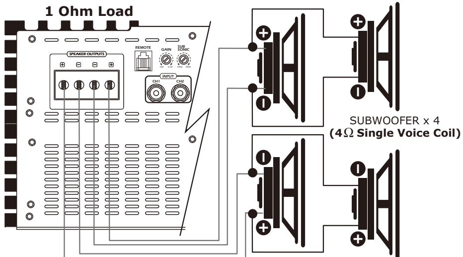
SUBWOOFER (4 Ω Single Voice Coil)
