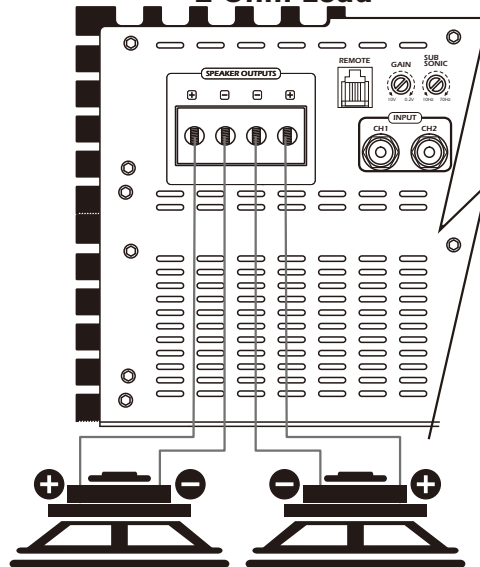
SUBWOOFER x 2 (4 Ω Single Voice Coil)
